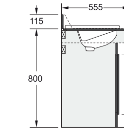
CV3 Profile Fully inset basin with upstand.
