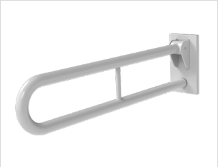
800mm hinged grab rail Powder coated stainless steel Doc M and HBN compliant 800mm hinged grab rail with concealed fixings. W800 x Ø35mm Code: White GRAB203 Blue GRAB206 Light Grey GRAB209 Dark Grey GRAB212
