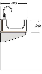
WT3 Thermo Slim Profile Slim thermoformed trough with deck mounted taps. A choice of brackets or underframe.
