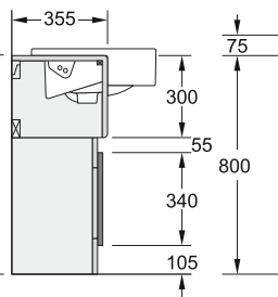
K2 Profile Semi-recessed basin without upstand.
