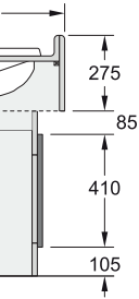
Baby Change Profile Fully inset basin with upstand.
