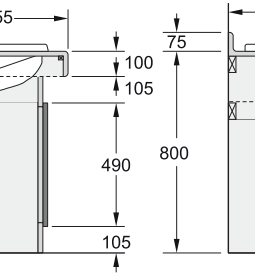
K4 Profile Fully inset basin without upstand.
