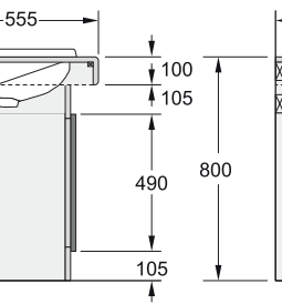
K3 Profile Fully inset basin with upstand.
